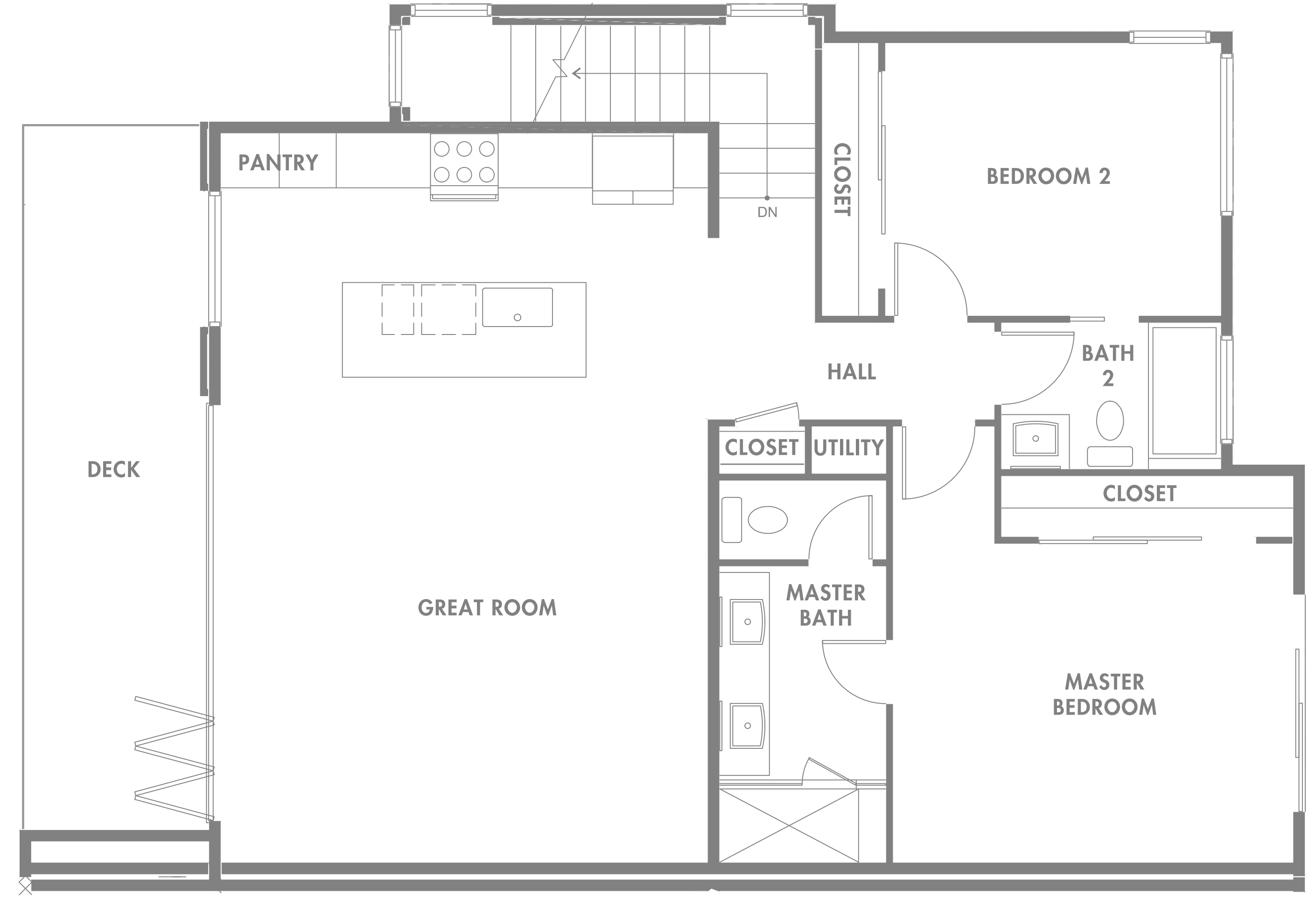
SECOND FLOOR
