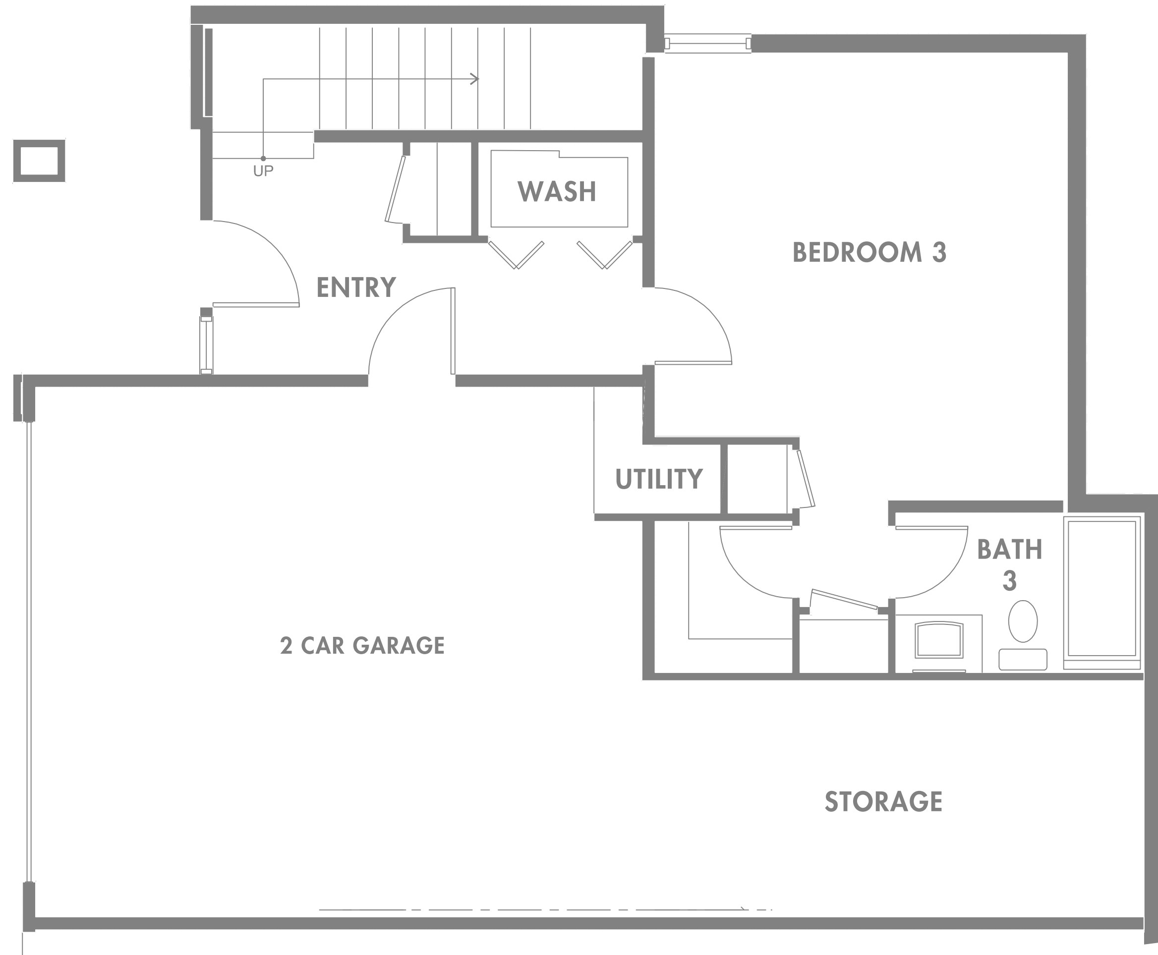
FIRST FLOOR
